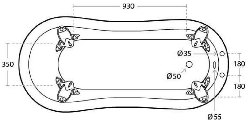
Bottom View
